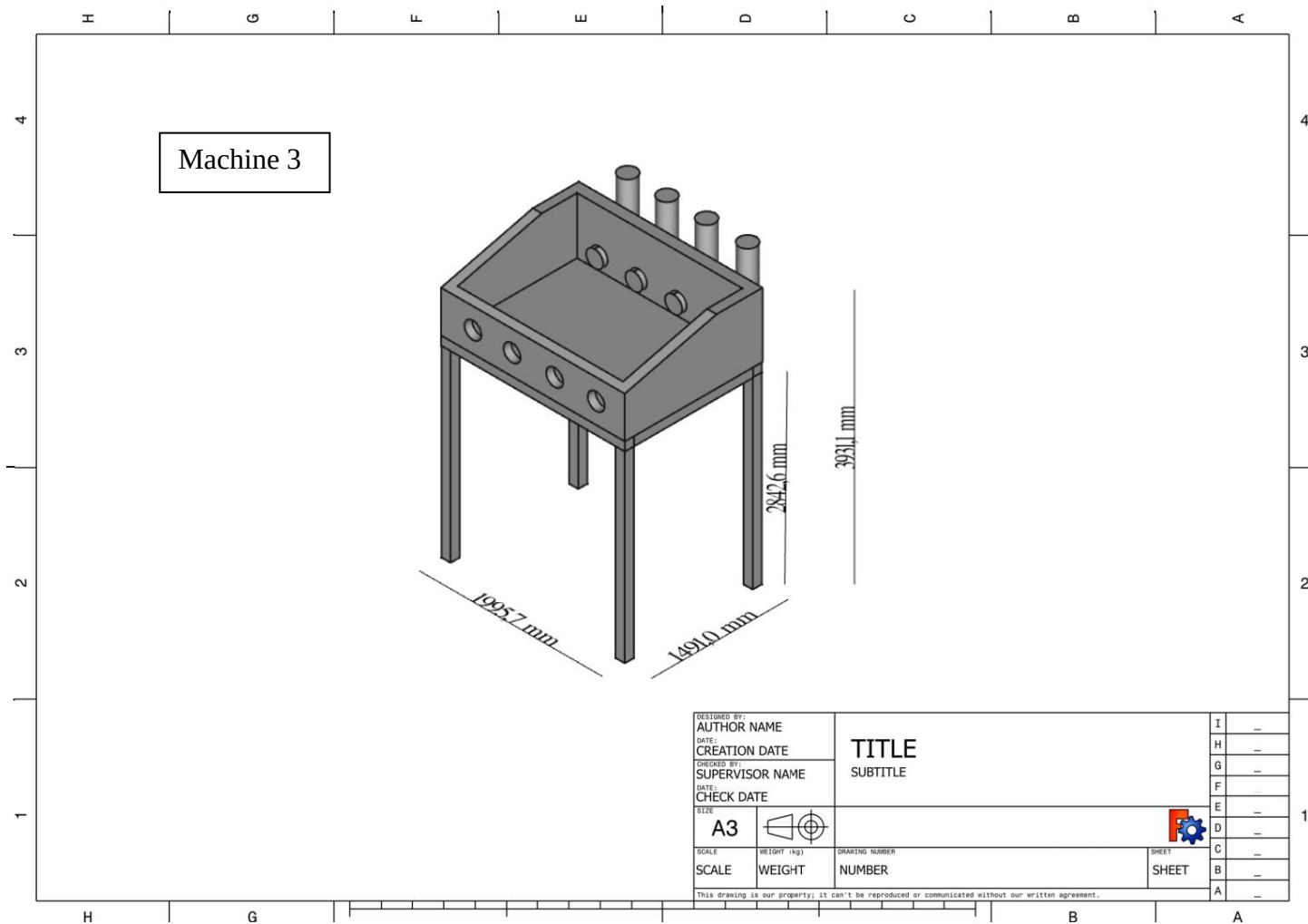
FIGURE 3. Isometric views of the MATILDA v1.0 prototype (the different machines are indicated). It was used FreeCAD v0.15 software (FreeCAD, 2015)
